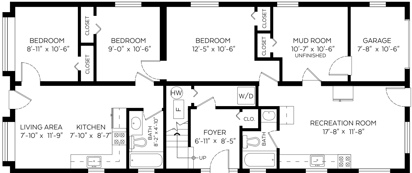
Lower Floor Plan Floor Area: 1,148 sq.ft
